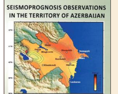
SEISMOPROGNOSIS OBSERVATIONS IN THE TERRITORY OF AZERBAIJAN
